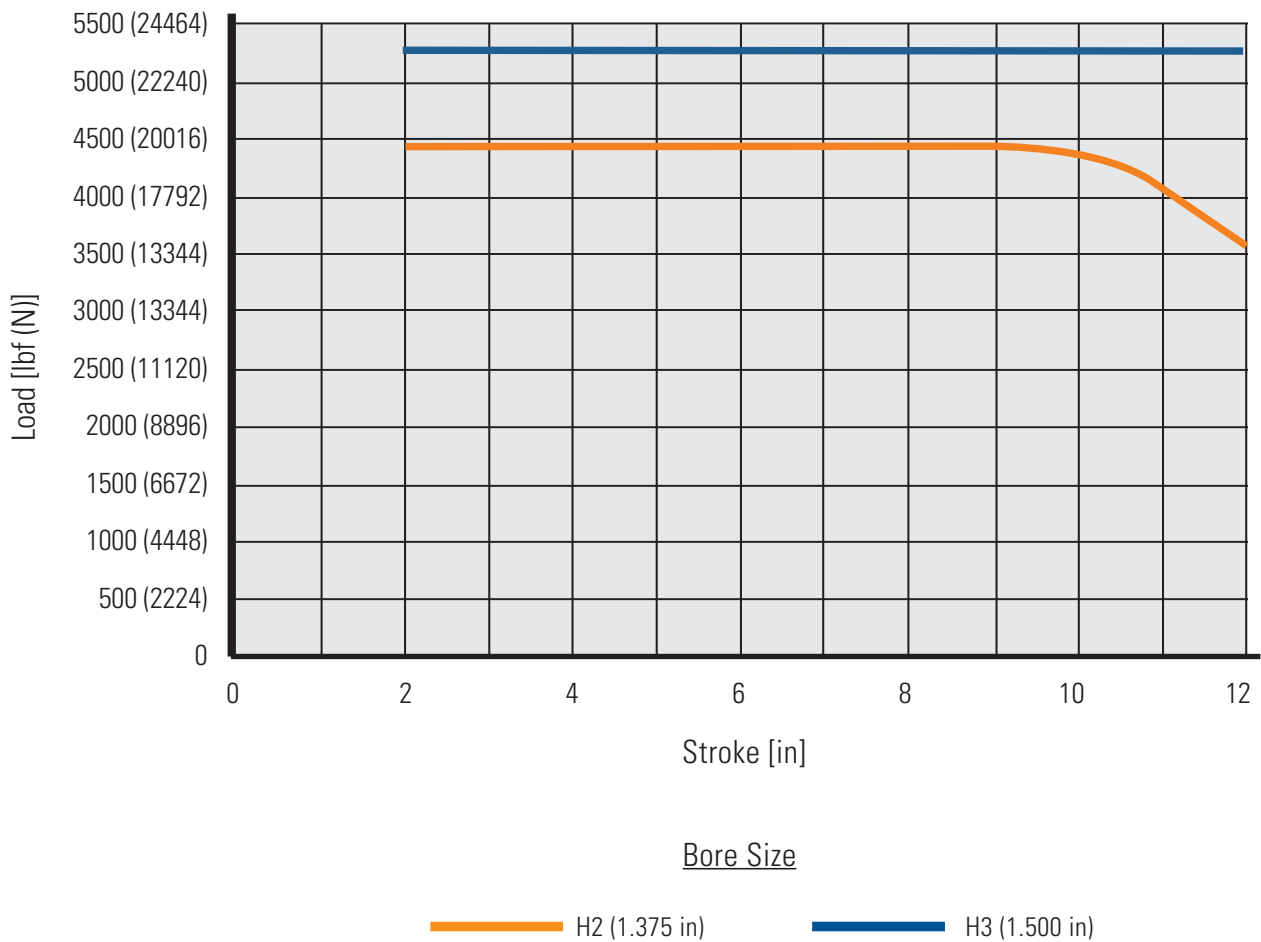
Stroke vs. Load and Bore Size
